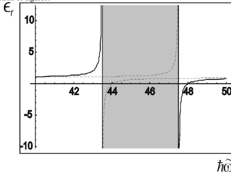
Figure 1. Dependence of dielectric permittivity on energy (frequency) of external field for bulk structures.
