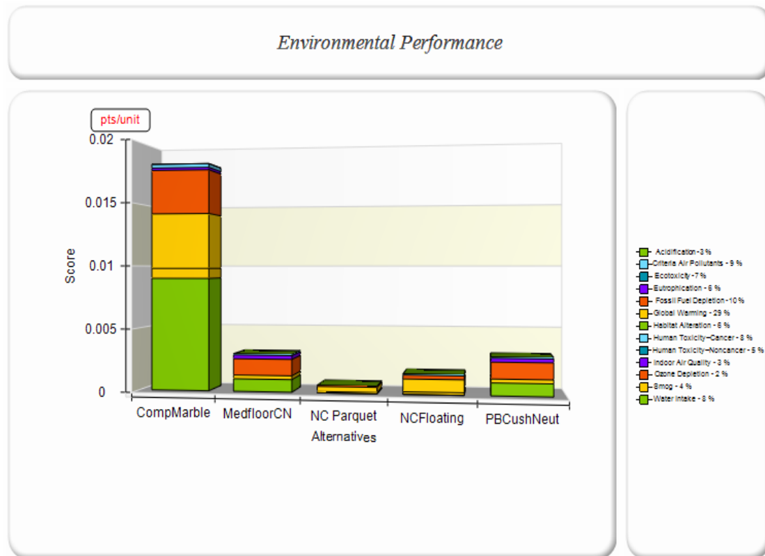
Chart 5. Comparison of total environmental performance of flooring
